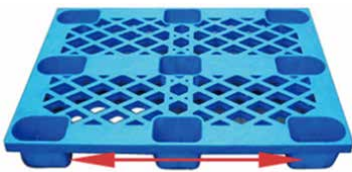
If the pallet spacing is larger than 700mm , select 685mm .
